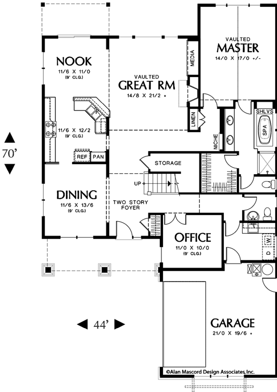
HOUSEPLAN 2.003 MAIN LEVEL FLOOR PLAN 1879 SQ FT
